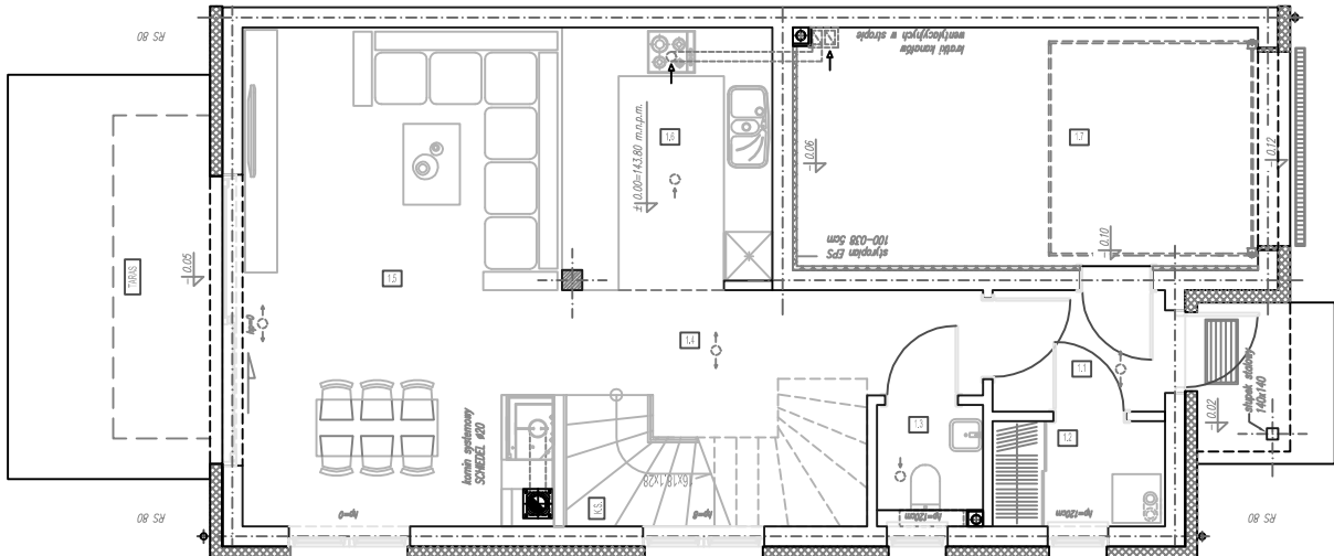
PARTER
